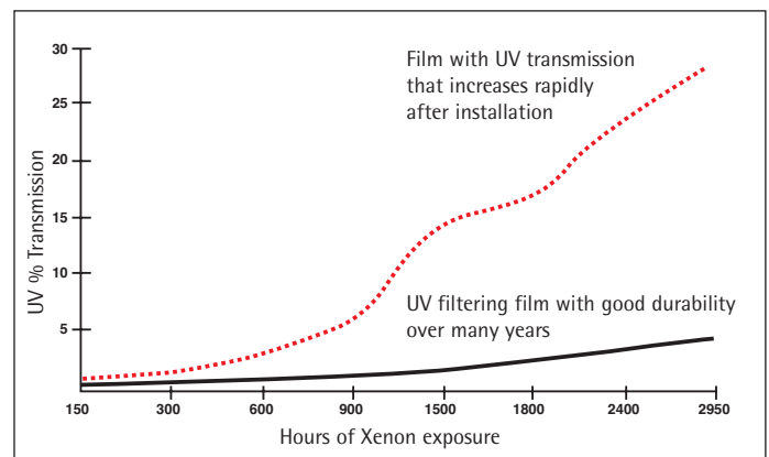
Figure 2: UV Transmission % of UV filtering window films with accelerated ageing
